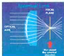
Spherical aberration causes a soft image, and requires multiple spherical elements to correct.
