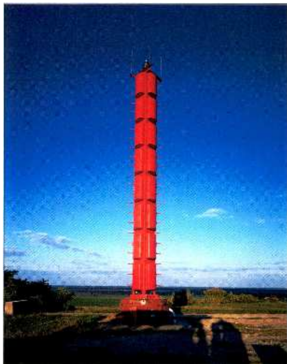
This Harris TAD-16UDA UHF Deltawing antenna is shown on the company's test range near Palmyra, MO.
