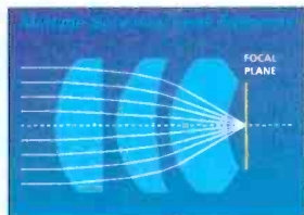
Spherical aberration causes a soft image, and requires multiple spherical elements to correct.
